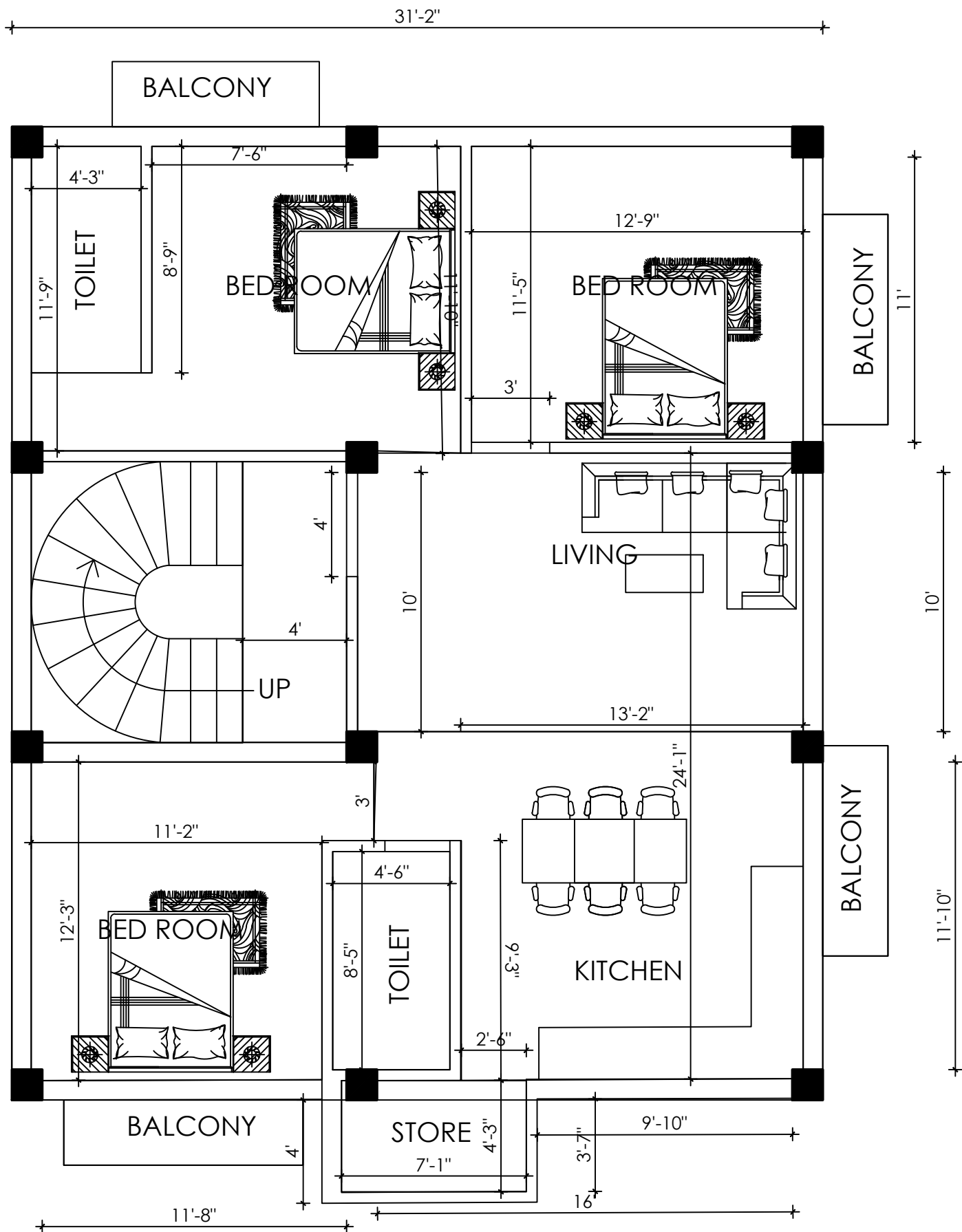
FIRST FLOOR PLAN AREA = 1100 SQ.FT
